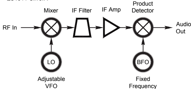
Figure A — Simplified block diagram of a superheterodyne receiver. Tuning the VFO of the receiver varies the frequency of the local oscillator (LO) so that the received RF signal appears to vary in frequency within the IF filter passband. This changes the audio frequency produced by the product detector.
