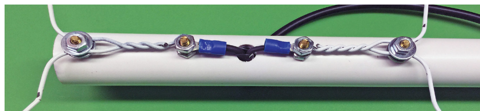
Figure 4 — Closeup of the feed point and hanger mounting.
